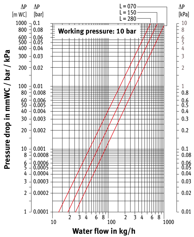
PRESSURE DROP TYPE 11
