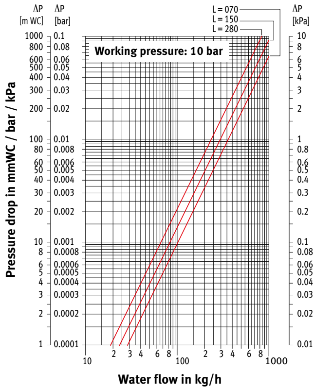
PRESSURE DROP TYPE 10
