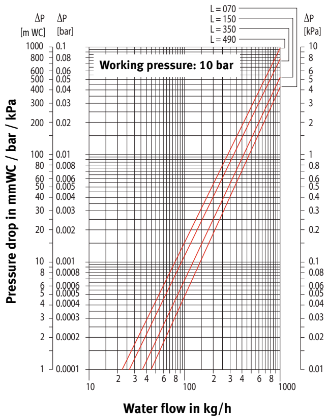
PRESSURE DROP TYPE 10
