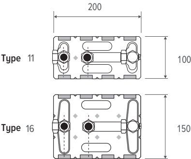
BOTTOM VIEW (in mm)
