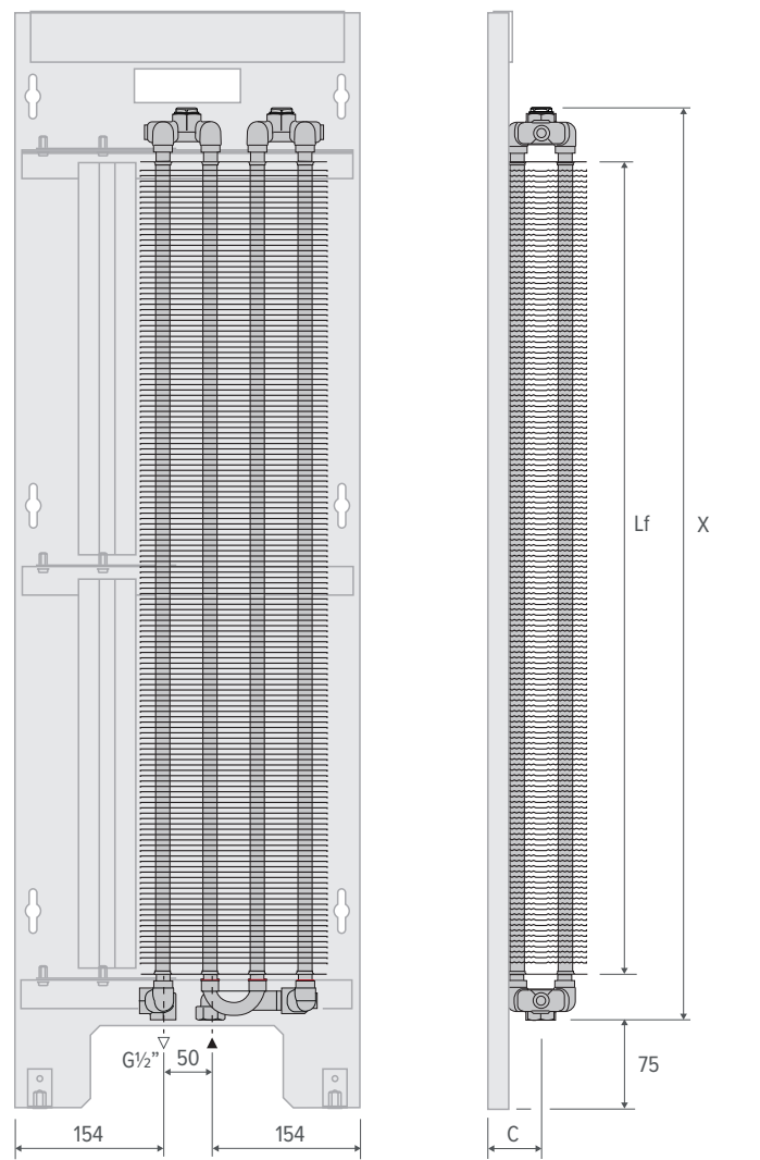
FRONT VIEW & SIDE VIEW (in mm)
