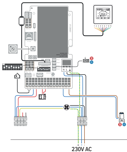
2-PIPE
