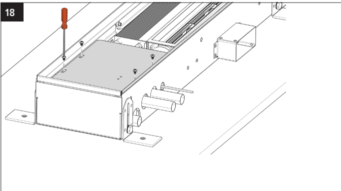
Mount the valve cover plate. Cover the casing with the protection foil and the protective cover.
