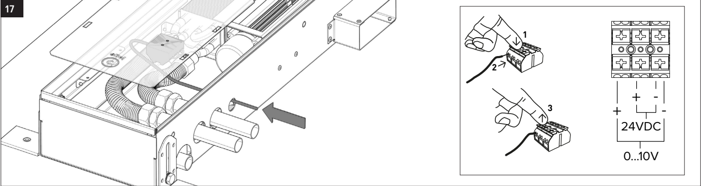
On the side of the hydronic connection, you can also find the terminal block for the electrical connection. The electrical connection is connected to the black block at the base of the protective cover.
