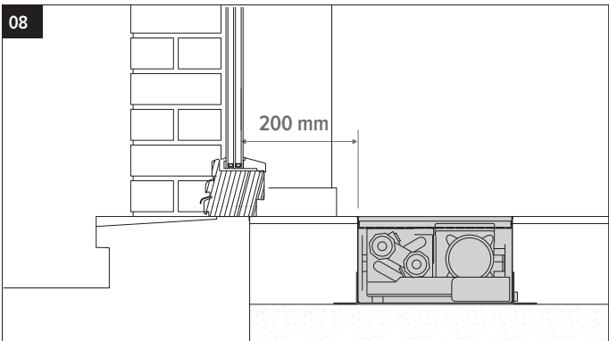
Install the device with the coil facing the wall or window.
