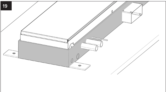
If screed is used the device needs to be completely insulated in order to protect the device from voltage differences.
