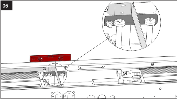
Make sure that the units are positioned correctly and that the casings fit tightly. Use the supplied connecting pieces to connect the different units.
