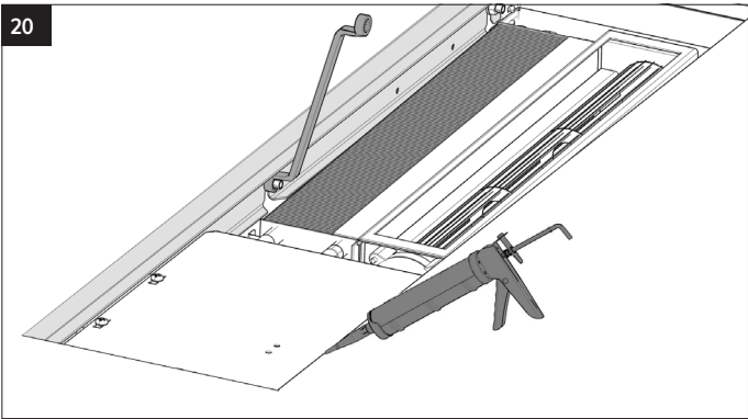
Fine adjustment to max. 0.8 cm, for a perfect alignment with the finished floor. Apply the finishing touches.
